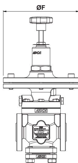
Fig. 1 - Valve with standard diaphragm
